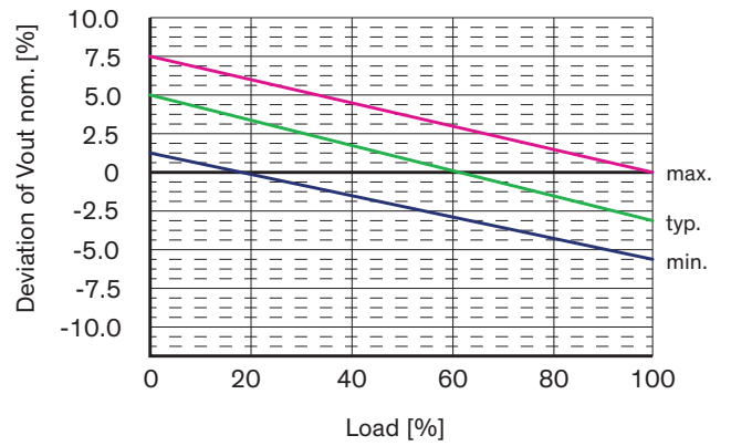
5 Vout models
